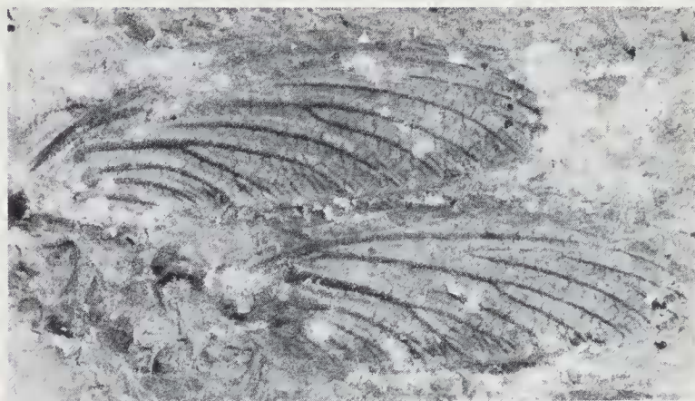
Figure 7. Protoreisma americana (Demoulin). Photograph of fore and hind wing-pads of holotype. The dark veins are convex, the weak ones (hardly visible) are concave. Length of fore wing-pad, 5.5 mm.
